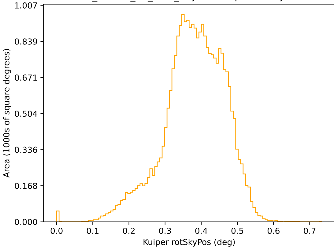
ddf_loaded_fl1_v3.4_10yrs r: Kuiper rotSkyPos
