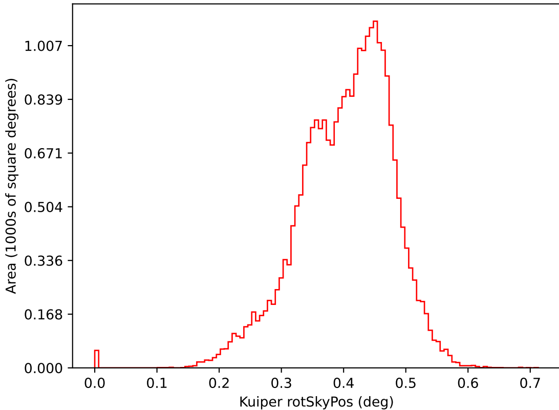
ddf_loaded_fl1_v3.4_10yrs i: Kuiper rotSkyPos
