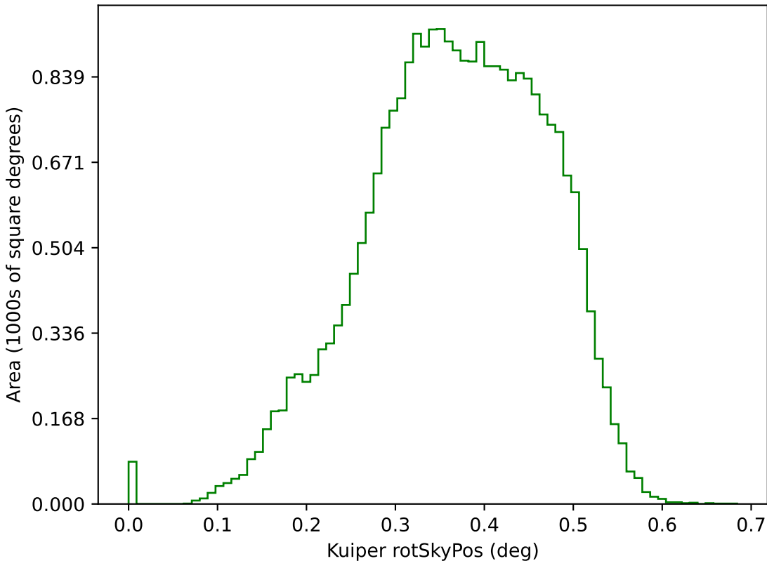
ddf_loaded_fl1_v3.4_10yrs g: Kuiper rotSkyPos
