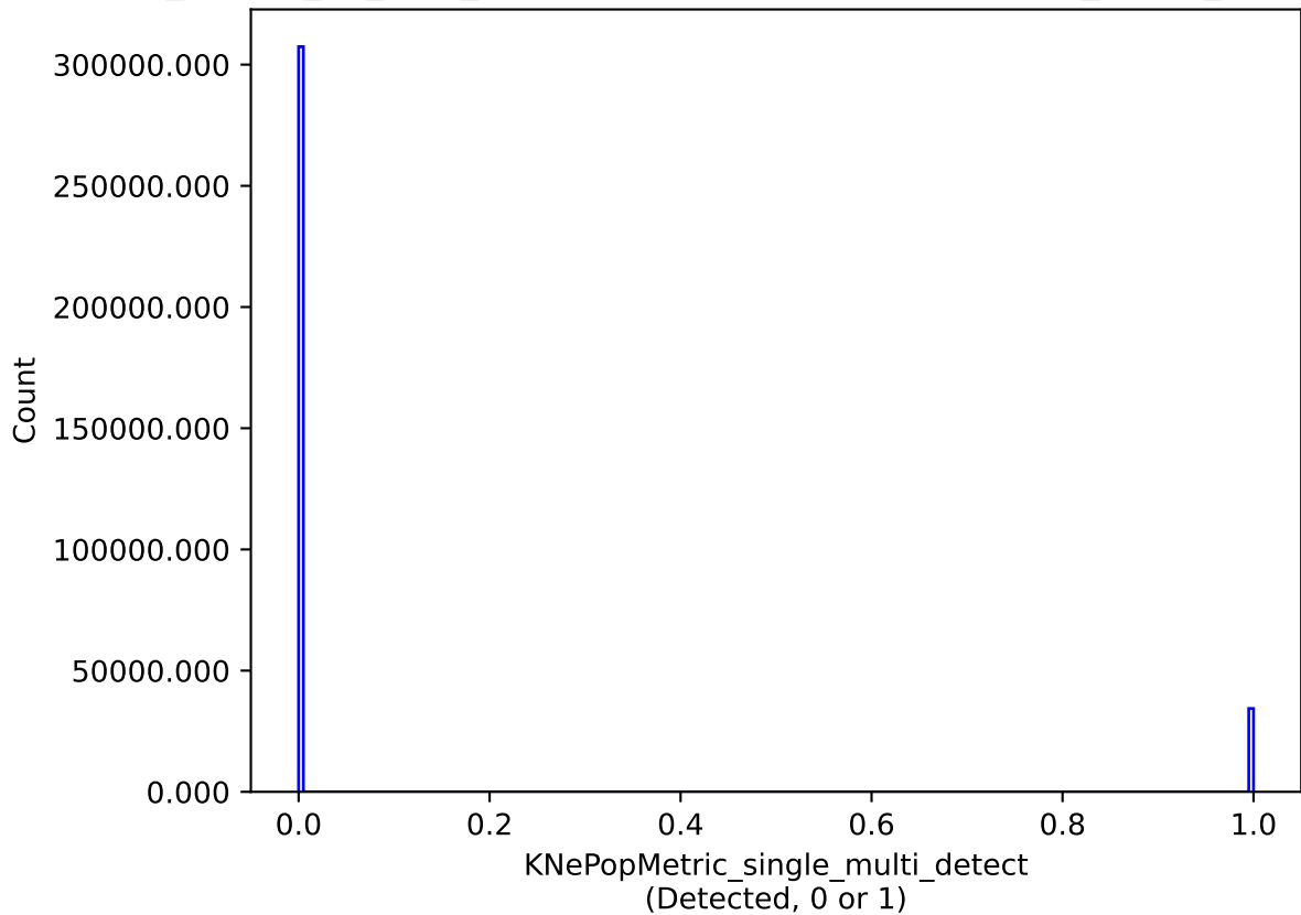
ddf_loaded_fl1_v3.4_10yrs single model: KNePopMetric_single_multi_detect
