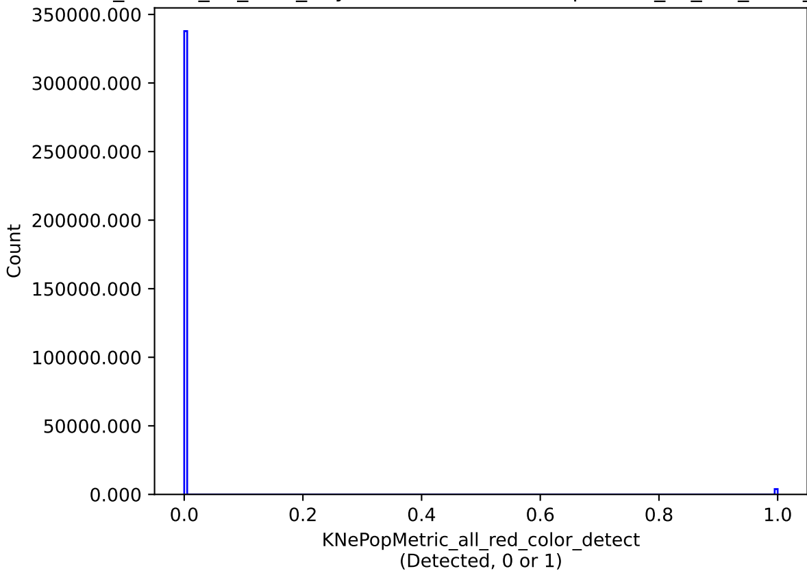
ddf_loaded_fl1_v3.4_10yrs all models: KNePopMetric_all_red_color_detect
