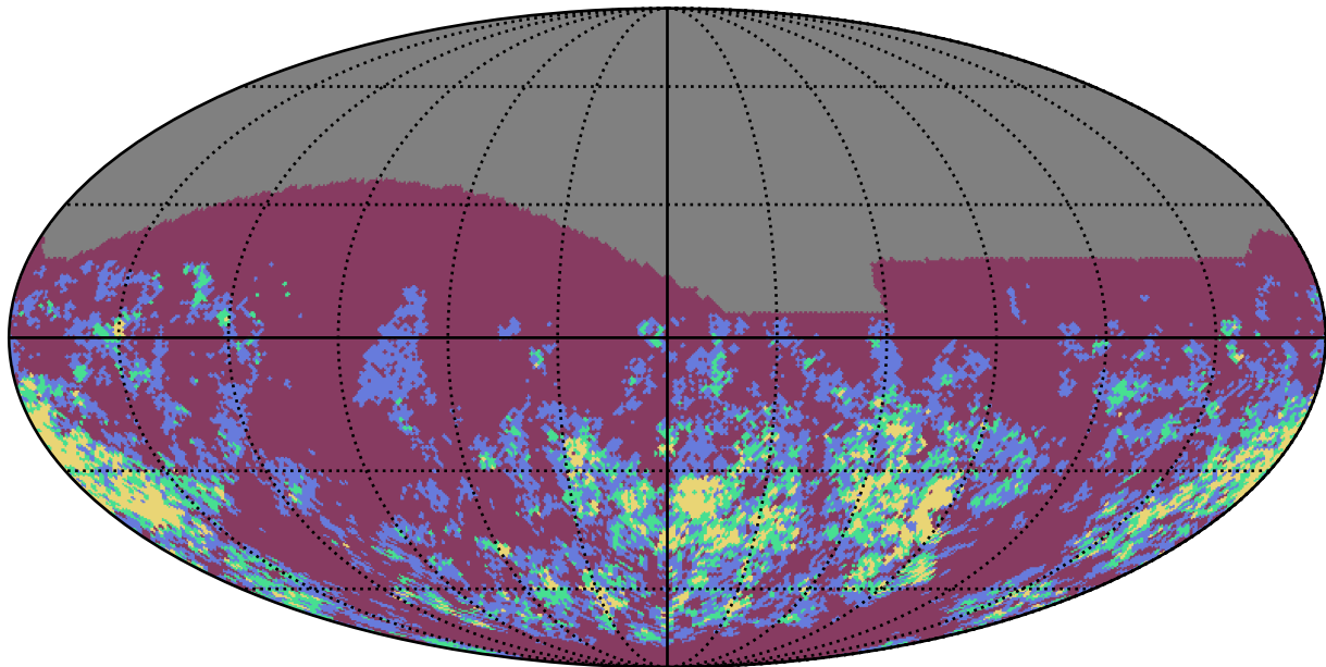
ddf_loaded_fl1_v3.4_10yrs z band: Gaps_7hr
