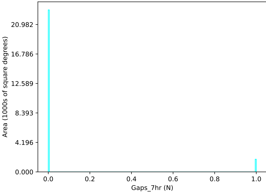
ddf_loaded_fl1_v3.4_10yrs u band: Gaps_7hr
