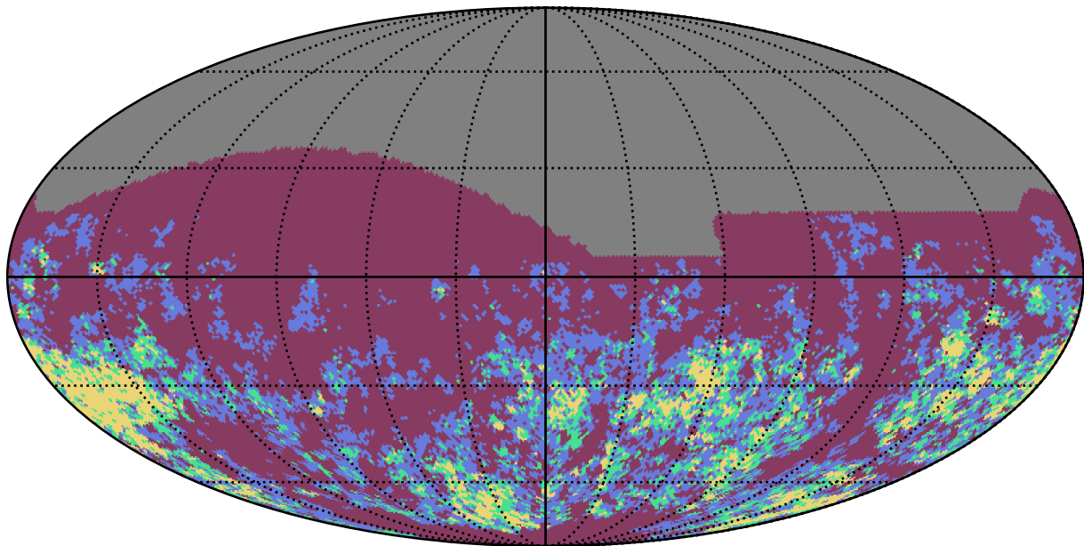
ddf_loaded_fl1_v3.4_10yrs i band: Gaps_7hr
