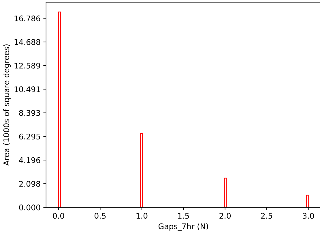
ddf_loaded_fl1_v3.4_10yrs i band: Gaps_7hr
