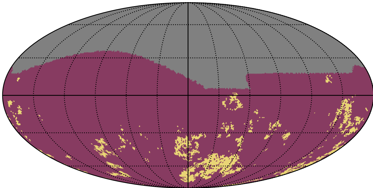
ddf_loaded_fl1_v3.4_10yrs g band: Gaps_7hr
