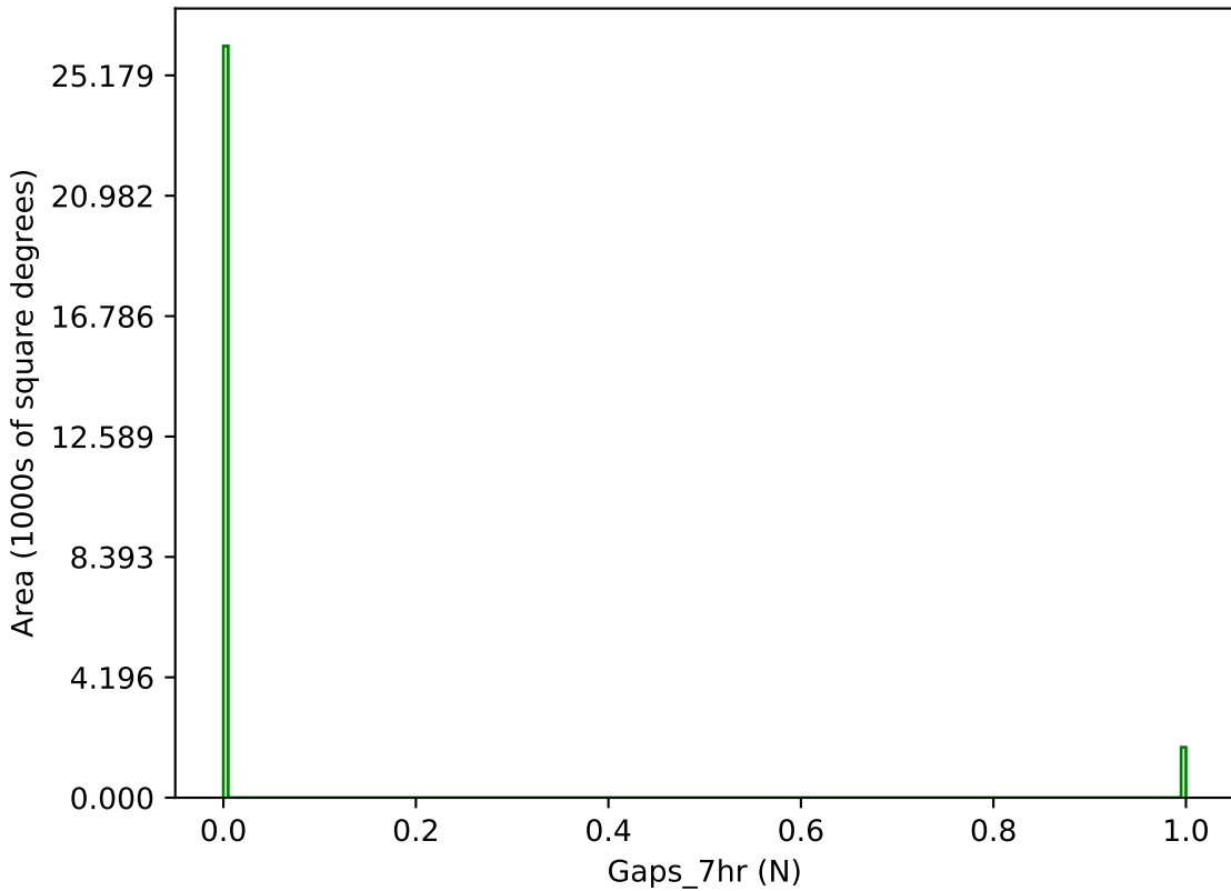
ddf_loaded_fl1_v3.4_10yrs g band: Gaps_7hr
