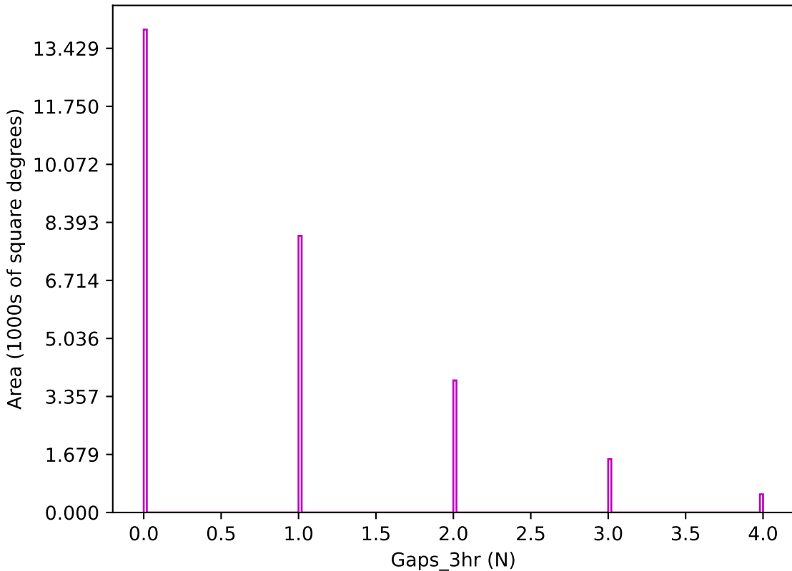
ddf_loaded_fl1_v3.4_10yrs z band: Gaps_3hr
