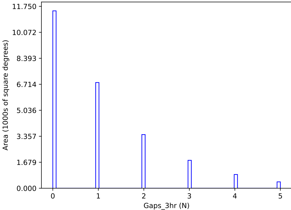
ddf_loaded_fl1_v3.4_10yrs y band: Gaps_3hr
