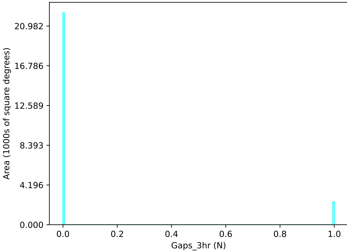
ddf_loaded_fl1_v3.4_10yrs u band: Gaps_3hr
