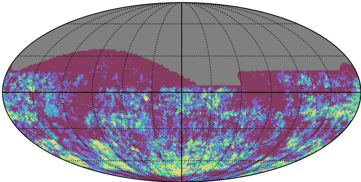
ddf_loaded_fl1_v3.4_10yrs i band: Gaps_3hr
