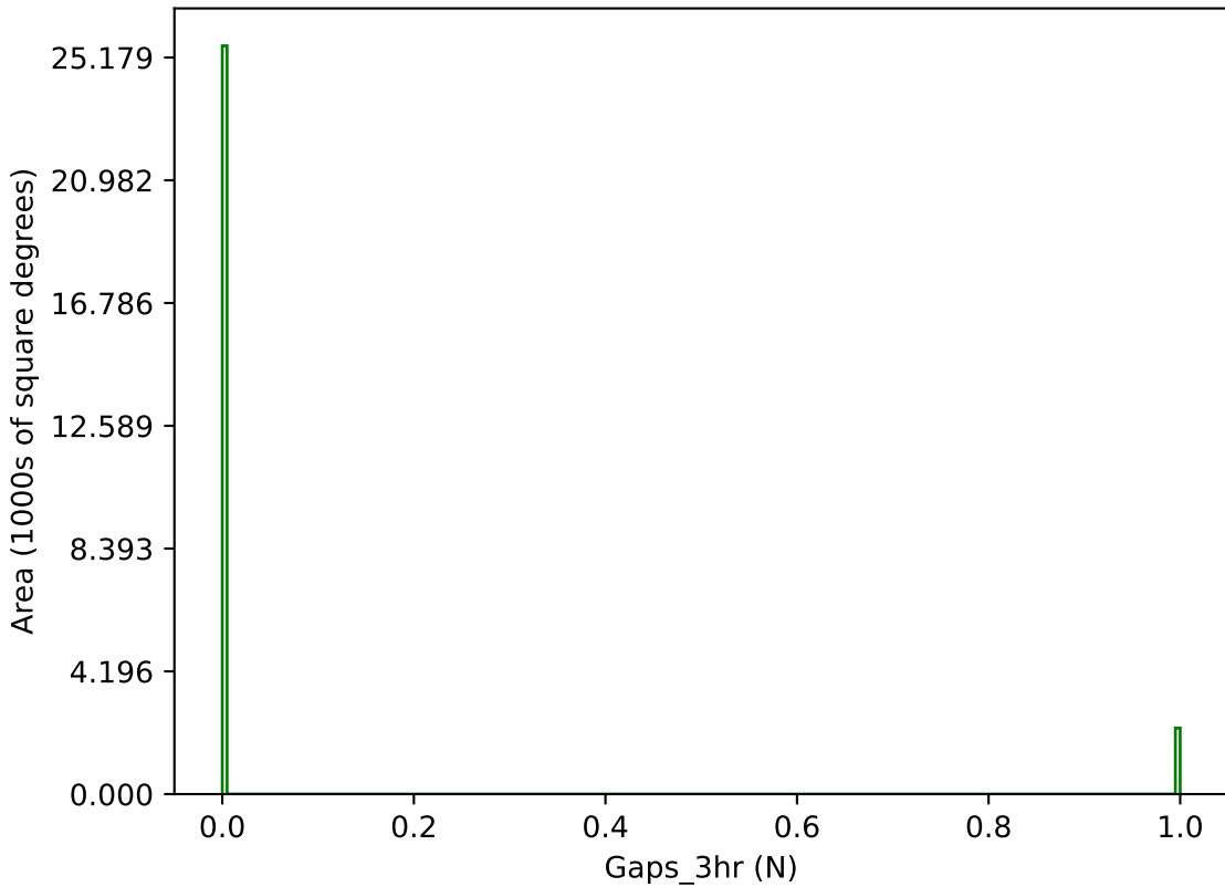
ddf_loaded_fl1_v3.4_10yrs g band: Gaps_3hr
