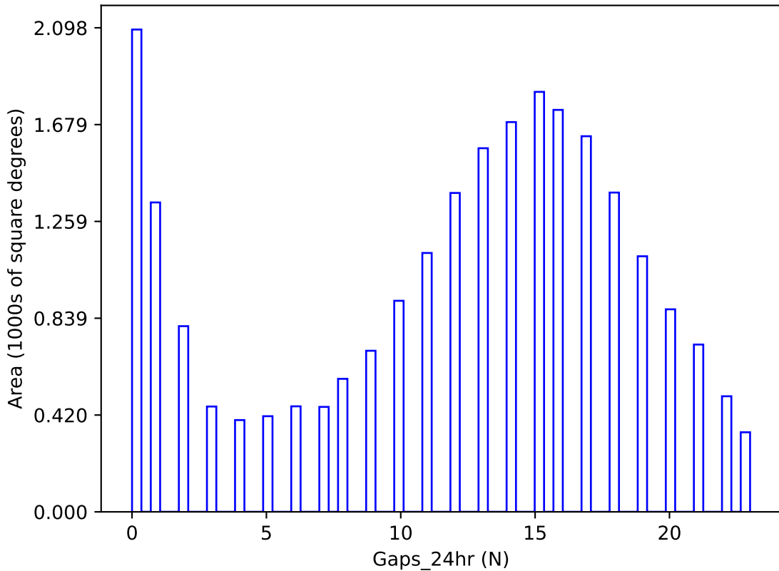
ddf_loaded_fl1_v3.4_10yrs y band: Gaps_24hr
