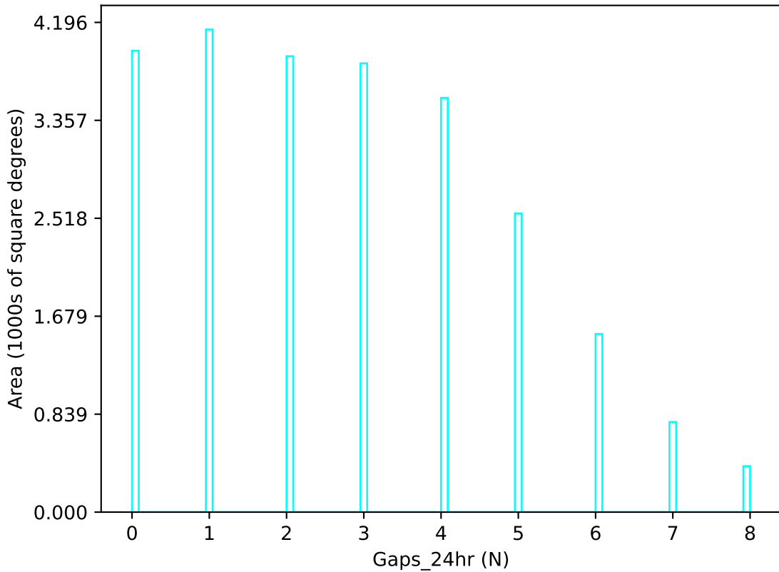
ddf_loaded_fl1_v3.4_10yrs u band: Gaps_24hr
