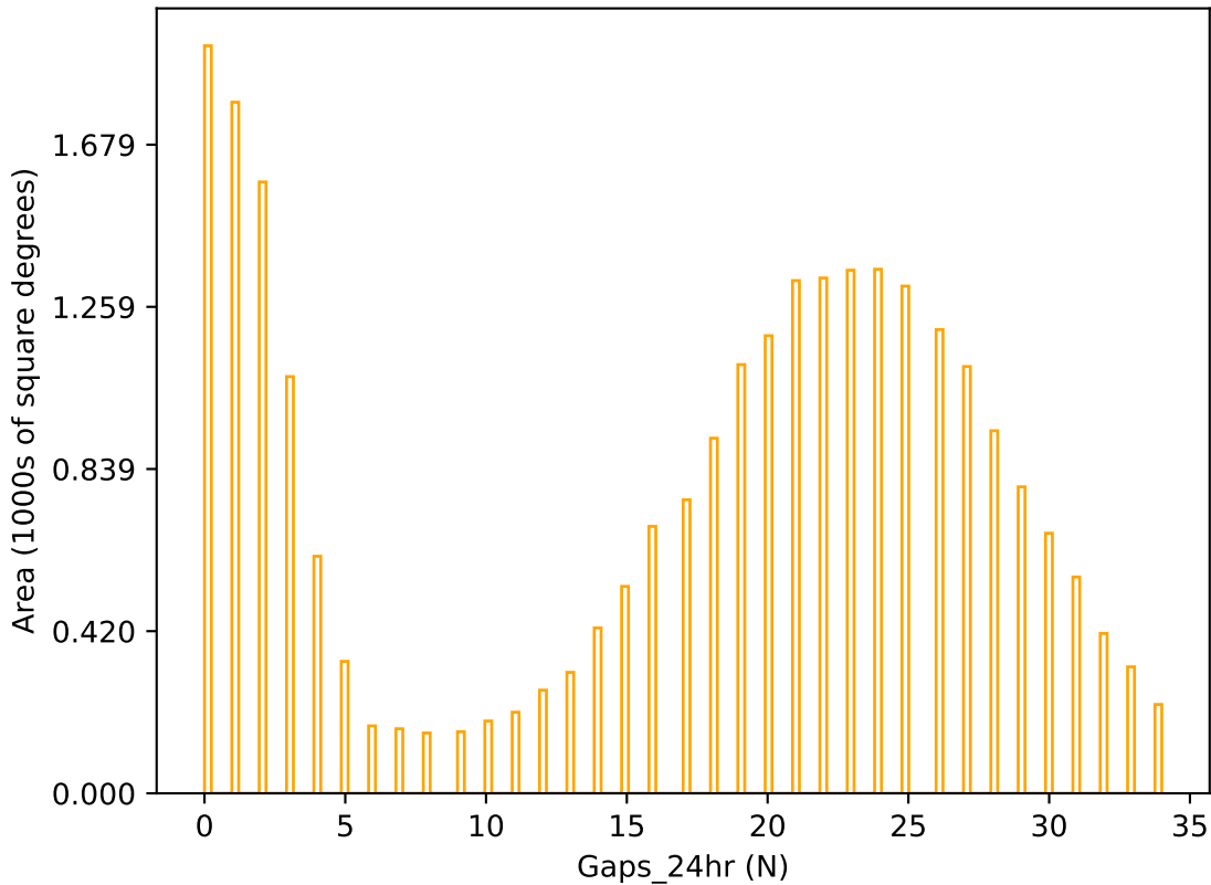
ddf_loaded_fl1_v3.4_10yrs r band: Gaps_24hr
