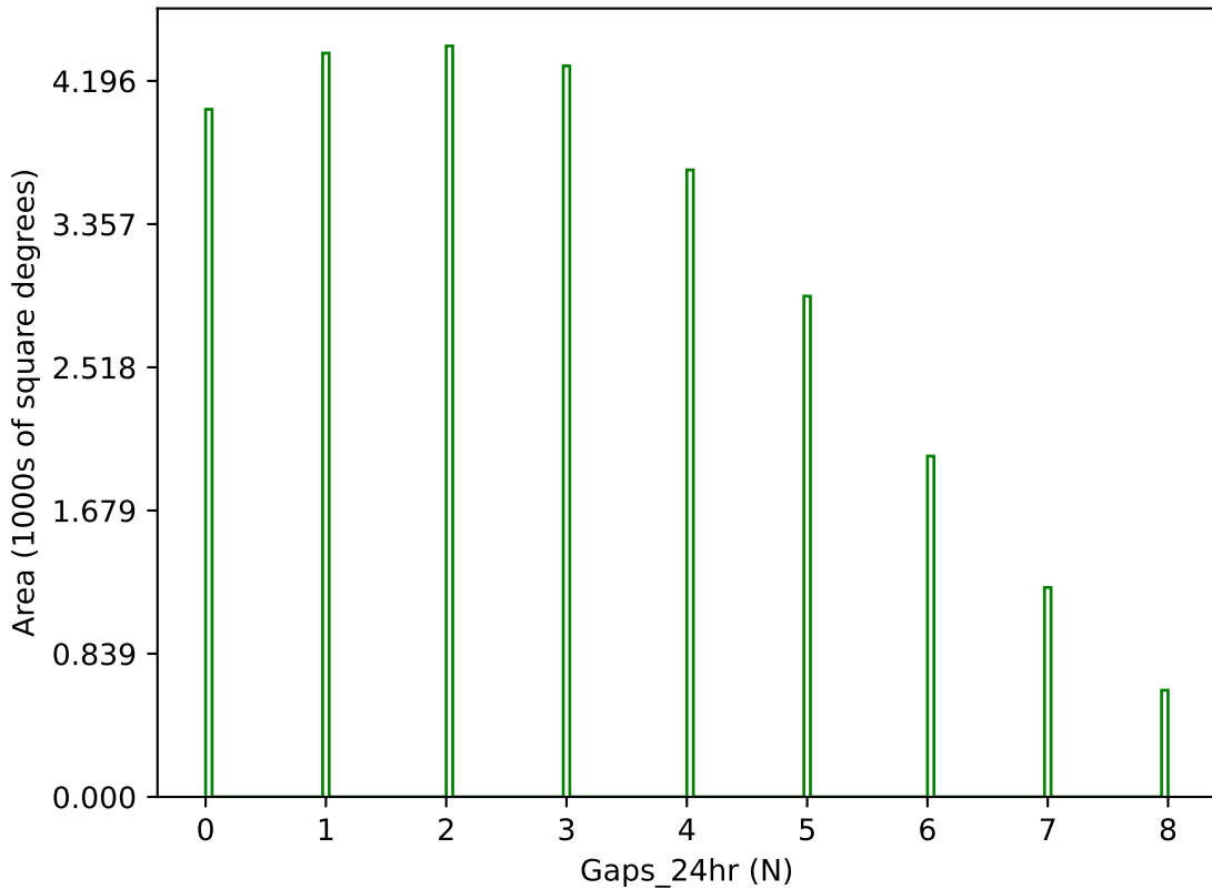
ddf_loaded_fl1_v3.4_10yrs g band: Gaps_24hr
