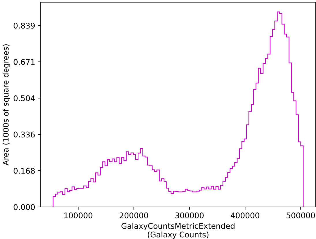
ddf_loaded_fl1_v3.4_10yrs z: GalaxyCountsMetricExtended
