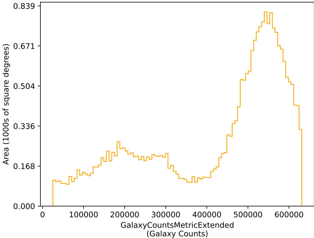
ddf_loaded_fl1_v3.4_10yrs r: GalaxyCountsMetricExtended
