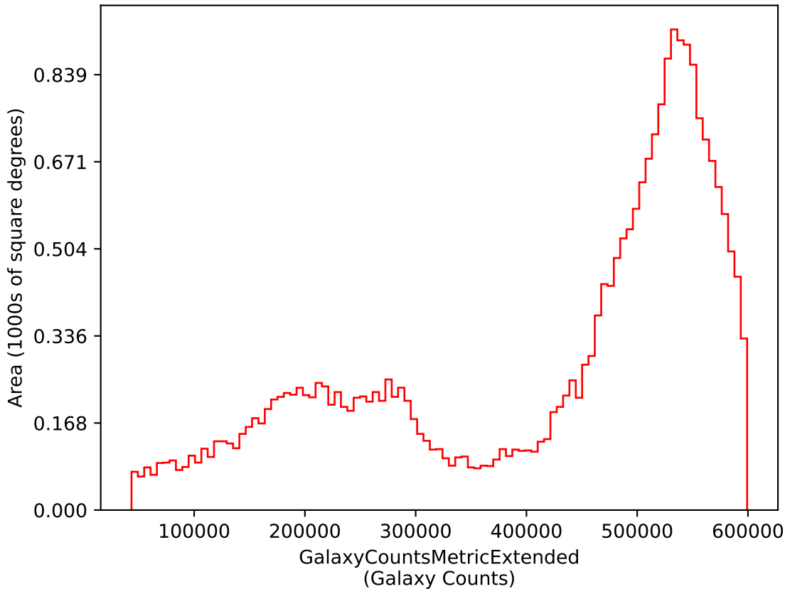
ddf_loaded_fl1_v3.4_10yrs i: GalaxyCountsMetricExtended
