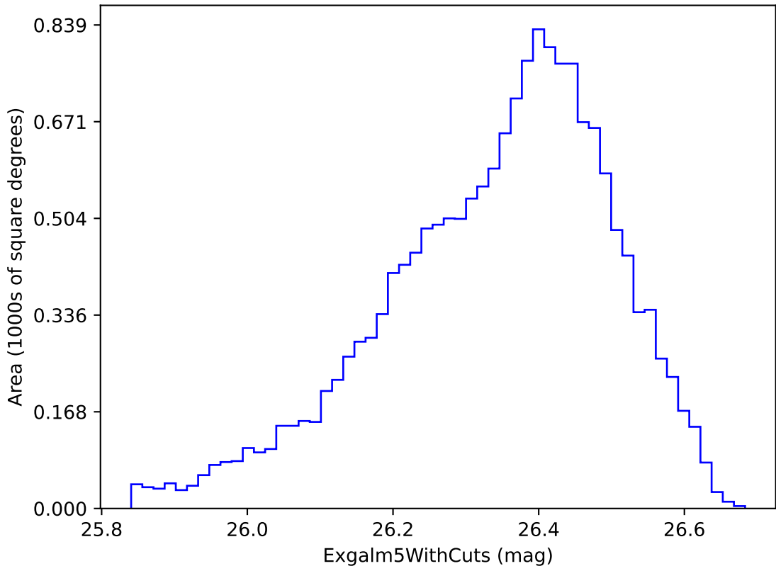
ddf_loaded_fl1_v3.4_10yrs i band non-DD year 9: ExgalM5WithCuts
