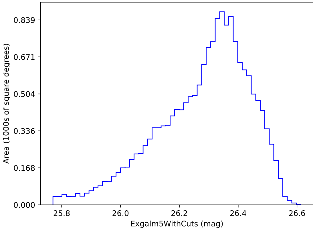
ddf_loaded_fl1_v3.4_10yrs i band non-DD year 8: ExgalM5WithCuts
