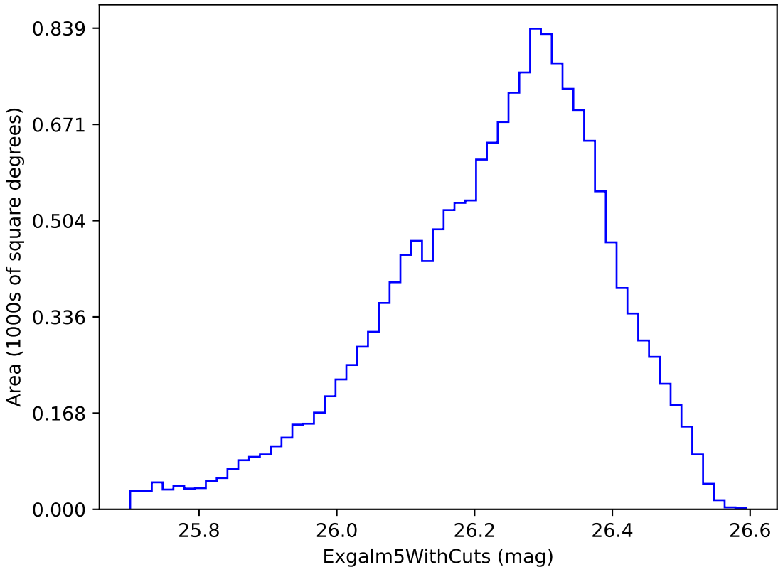
ddf_loaded_fl1_v3.4_10yrs i band non-DD year 7: ExgalM5WithCuts
