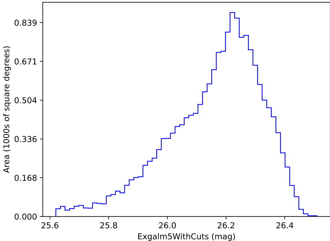
ddf_loaded_fl1_v3.4_10yrs i band non-DD year 6: ExgalM5WithCuts
