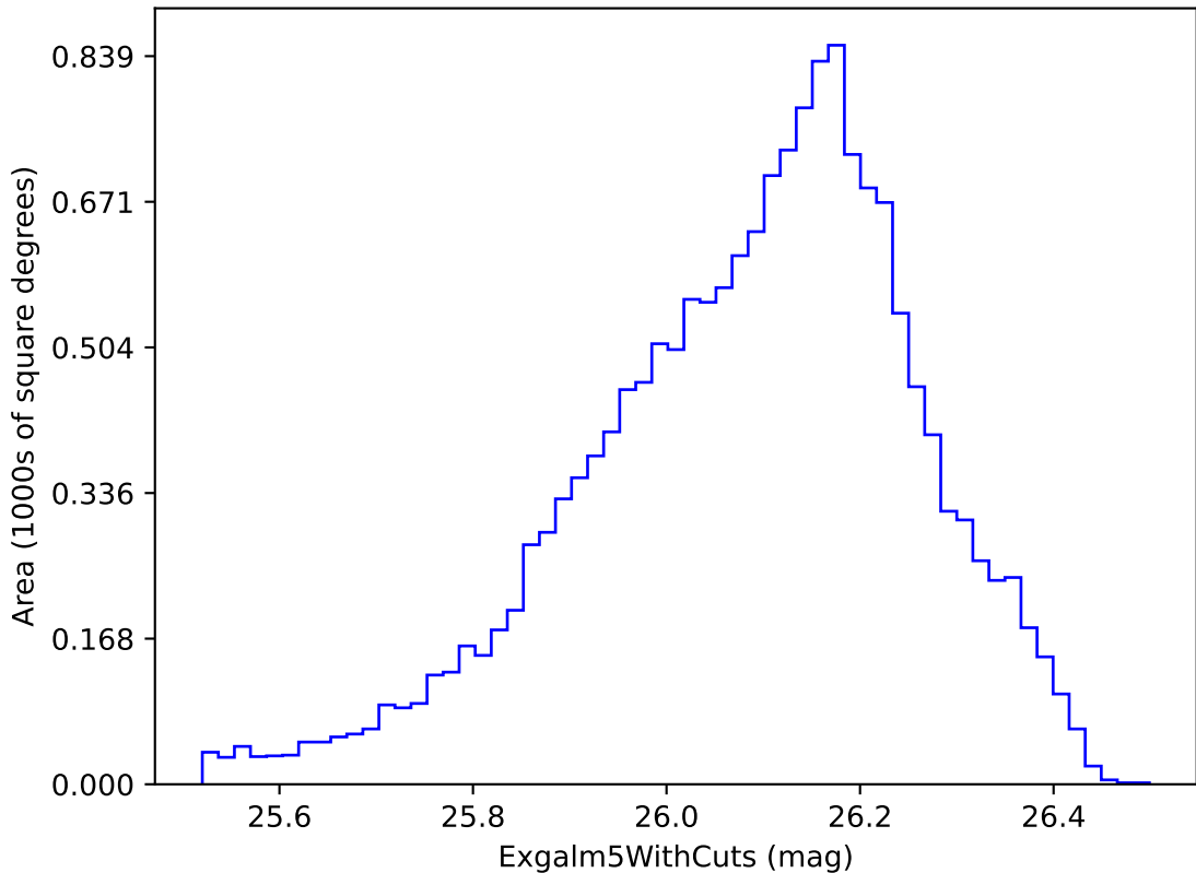
ddf_loaded_fl1_v3.4_10yrs i band non-DD year 5: ExgalM5WithCuts
