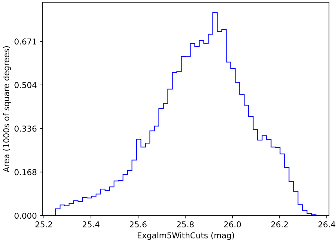
ddf_loaded_fl1_v3.4_10yrs i band non-DD year 3: Exgalml5WithCuts
