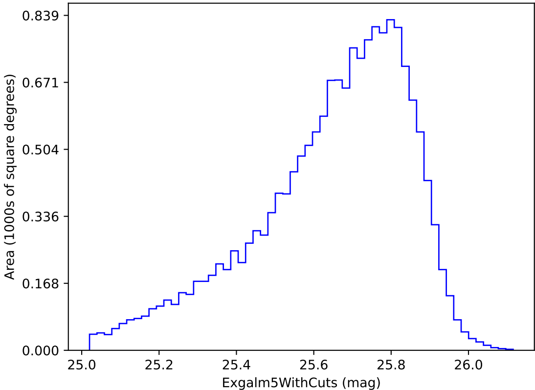
ddf_loaded_fl1_v3.4_10yrs i band non-DD year 2: Exgal5WithCuts
