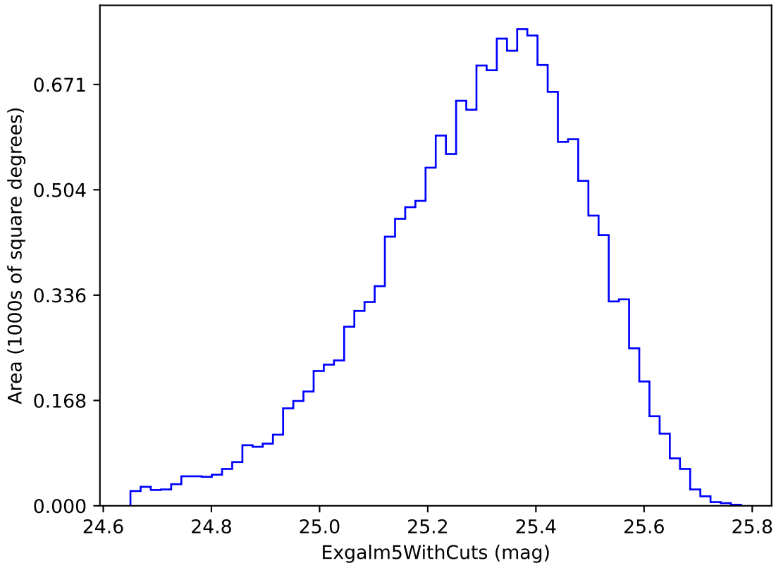
ddf_loaded_fl1_v3.4_10yrs i band non-DD year 1: Exgal5WithCuts
