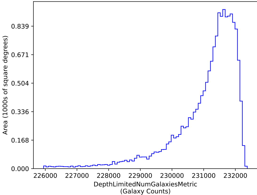
ddf_loaded_fl1_v3.4_10yrs i band galaxies non-DD: DepthLimitedNumGalaxiesMetric
