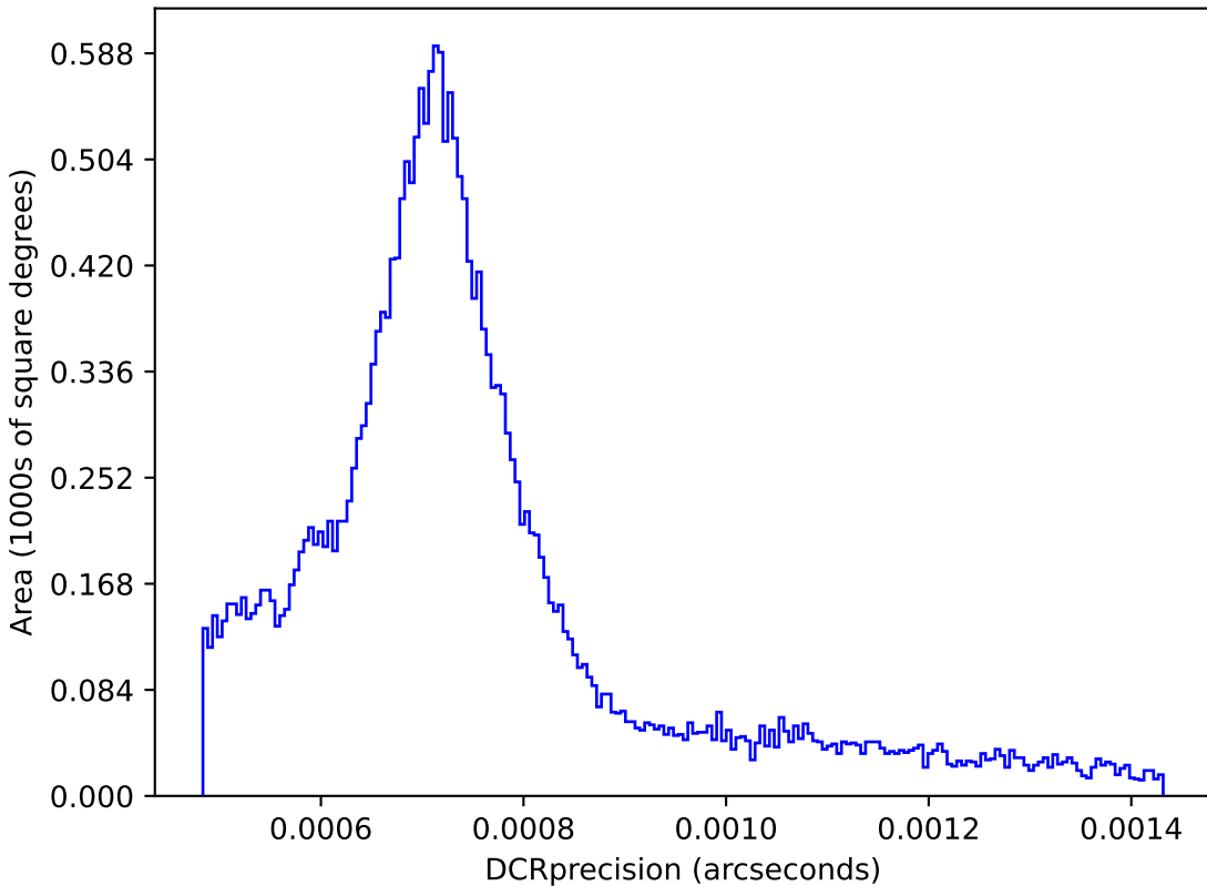
ddf_loaded_fl1_v3.4_10yrs : DCRprecision
