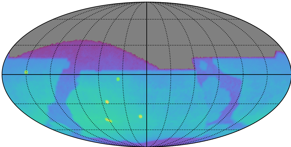
ddf_loaded_fl1_v3.4_10yrs : Brown Dwarf, L7
