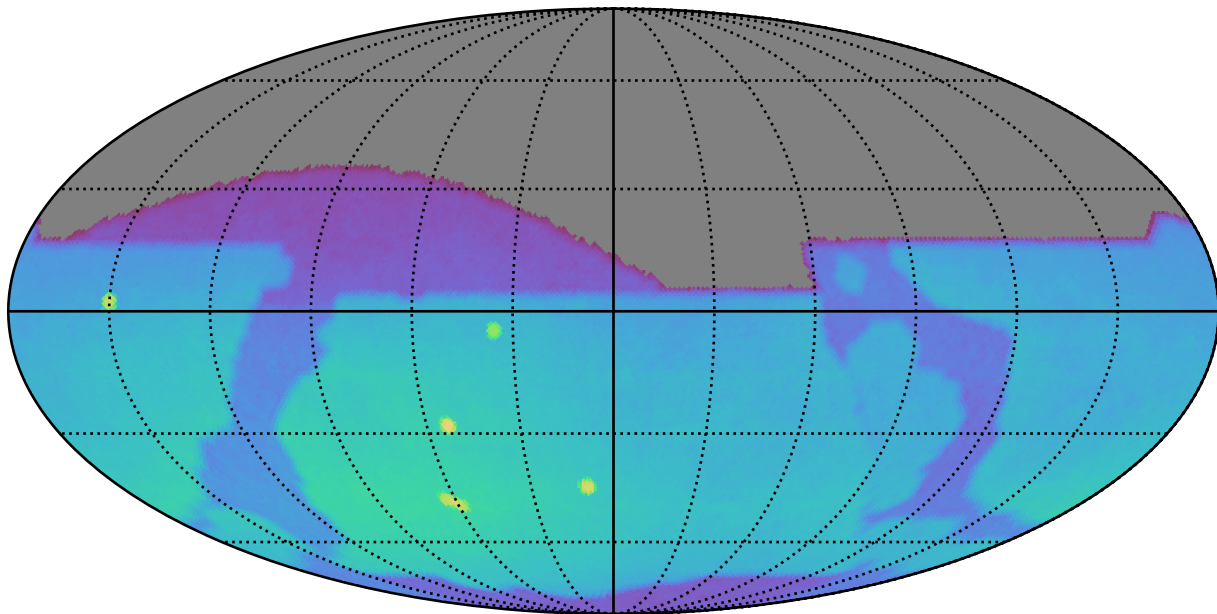
ddf_loaded_fl1_v3.4_10yrs : Brown Dwarf, L4
