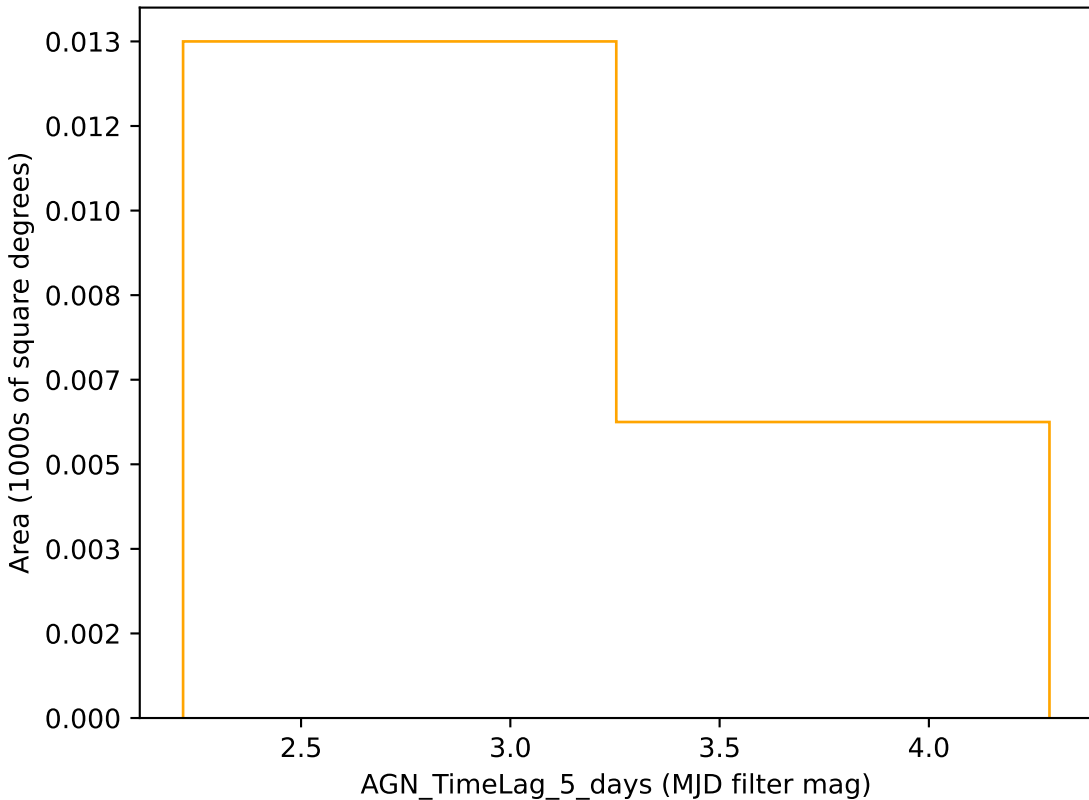
ddf_loaded_fl1_v3.4_10yrs r band: AGN_TimeLag_5_days
