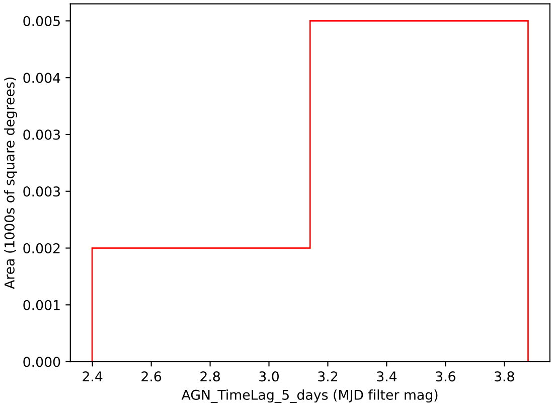
ddf_loaded_fl1_v3.4_10yrs i band: AGN_TimeLag_5_days
