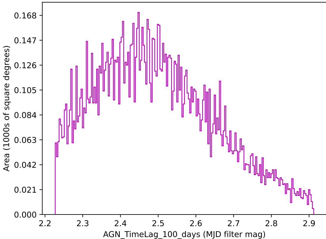
ddf_loaded_fl1_v3.4_10yrs z band: AGN_TimeLag_100_days
