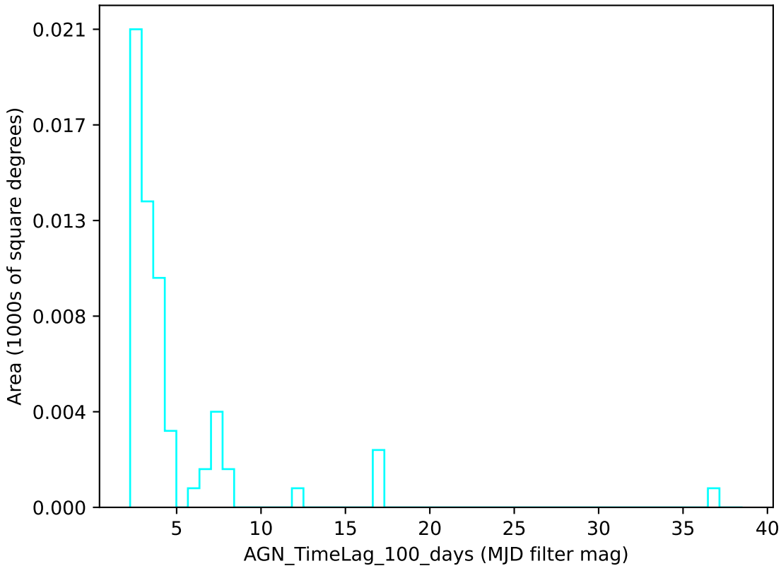
ddf_loaded_fl1_v3.4_10yrs u band: AGN_TimeLag_100_days
