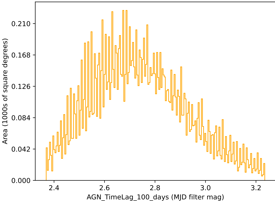
ddf_loaded_fl1_v3.4_10yrs r band: AGN_TimeLag_100_days
