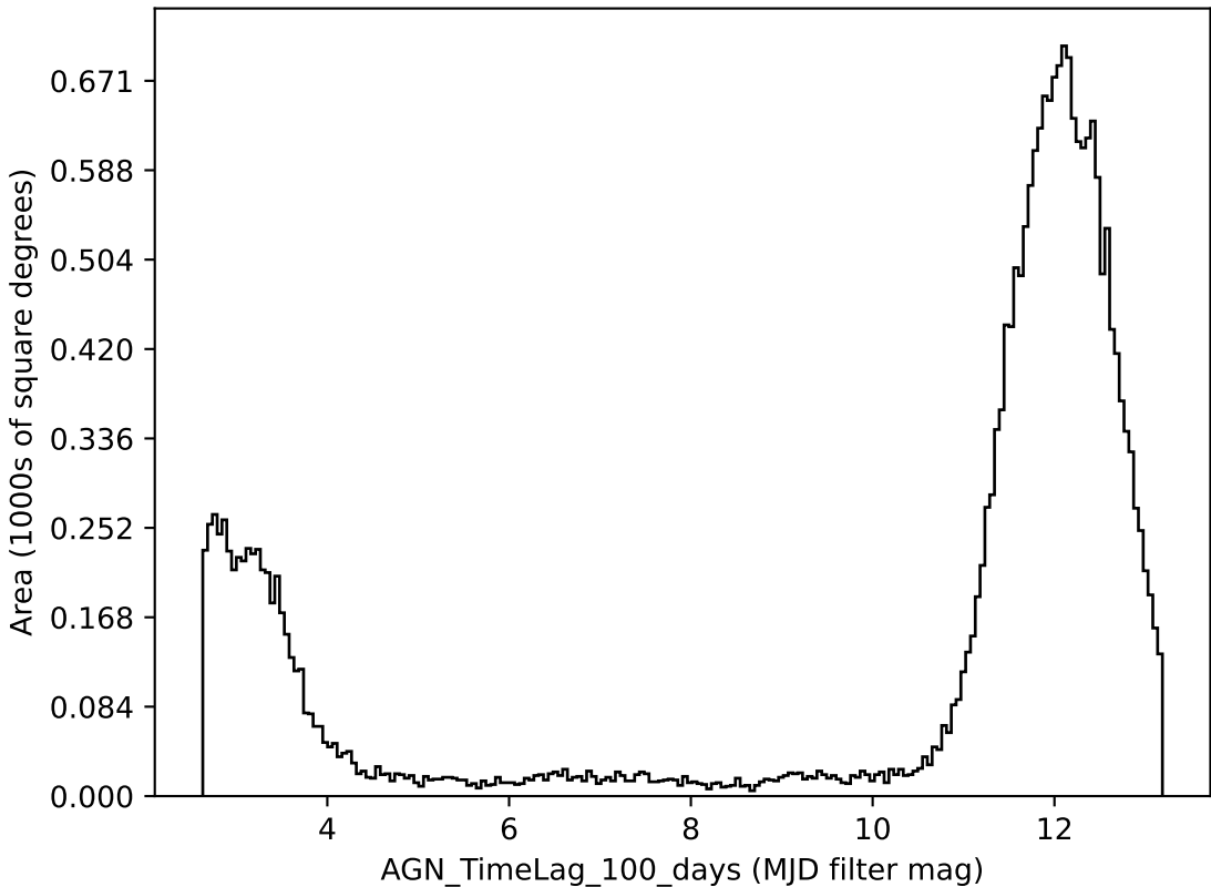
ddf_loaded_fl1_v3.4_10yrs all bands: AGN_TimeLag_100_days
