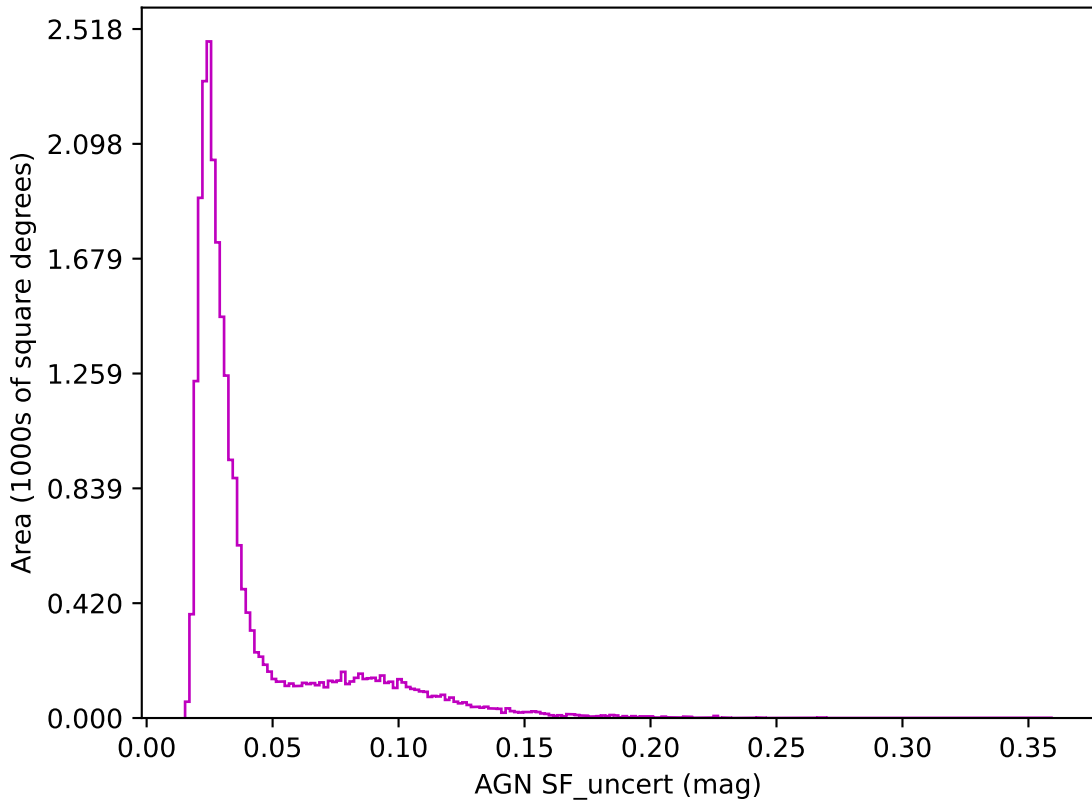
ddf_loaded_fl1_v3.4_10yrs z band: AGN SF_uncert
