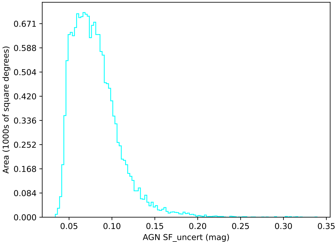
ddf_loaded_fl1_v3.4_10yrs u band: AGN SF_uncert
