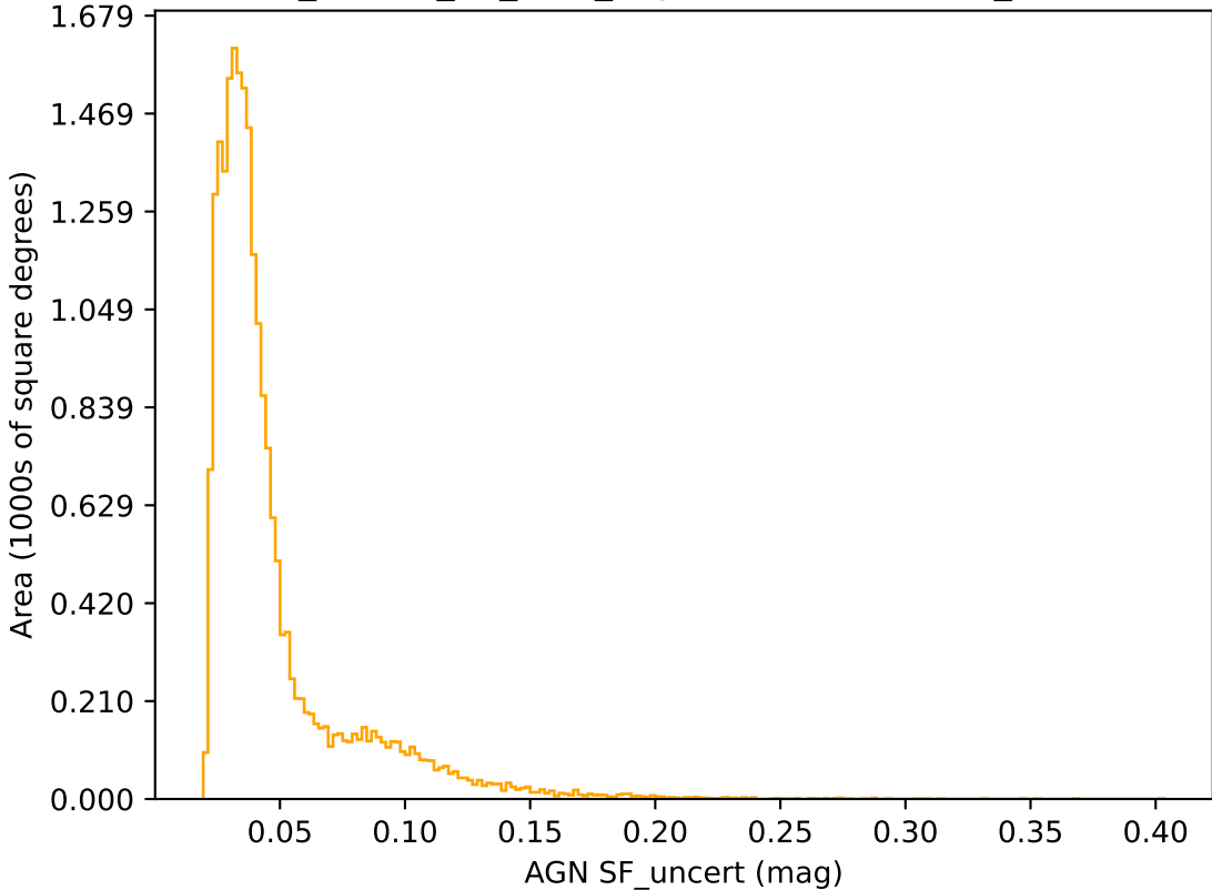
ddf_loaded_fl1_v3.4_10yrs r band: AGN SF_uncert
