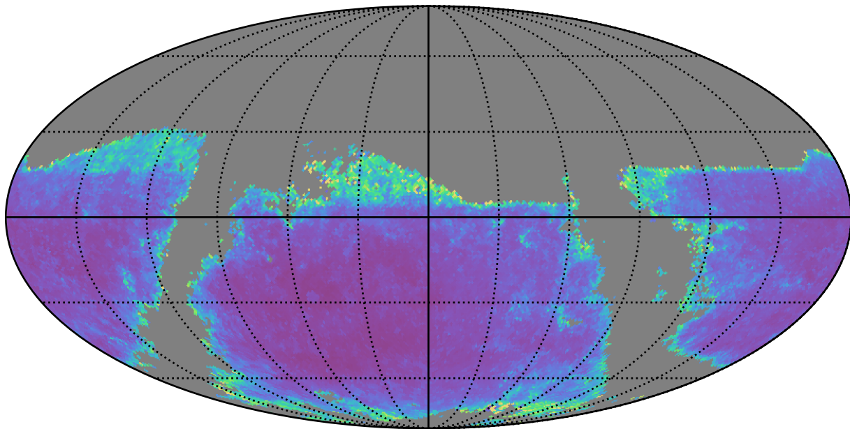
ddf_loaded_fl1_v3.4_10yrs g band: AGN SF_uncert
