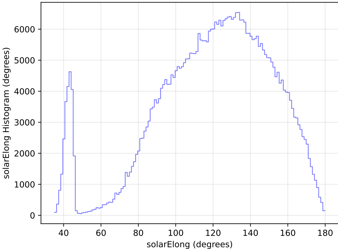
ddf_loaded_fl1_v3.4_10yrs WFD z band: solarElong Histogram
