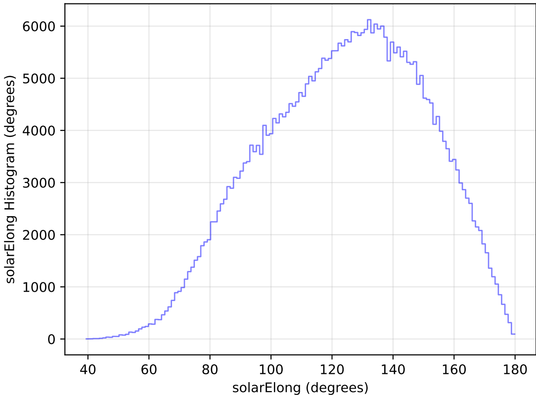
ddf_loaded_fl1_v3.4_10yrs WFD y band: solarElong Histogram
