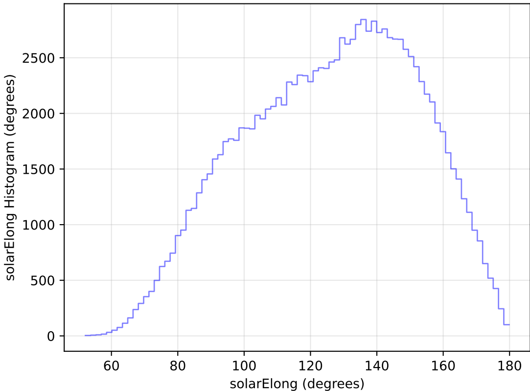
ddf_loaded_fl1_v3.4_10yrs WFD u band: solarElong Histogram
