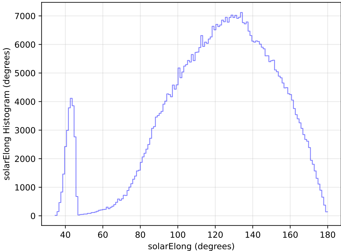
ddf_loaded_fl1_v3.4_10yrs WFD i band: solarElong Histogram
