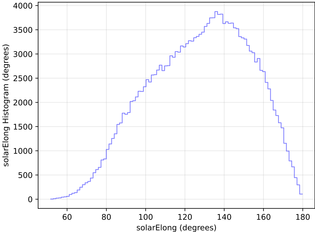
ddf_loaded_fl1_v3.4_10yrs WFD g band: solarElong Histogram
